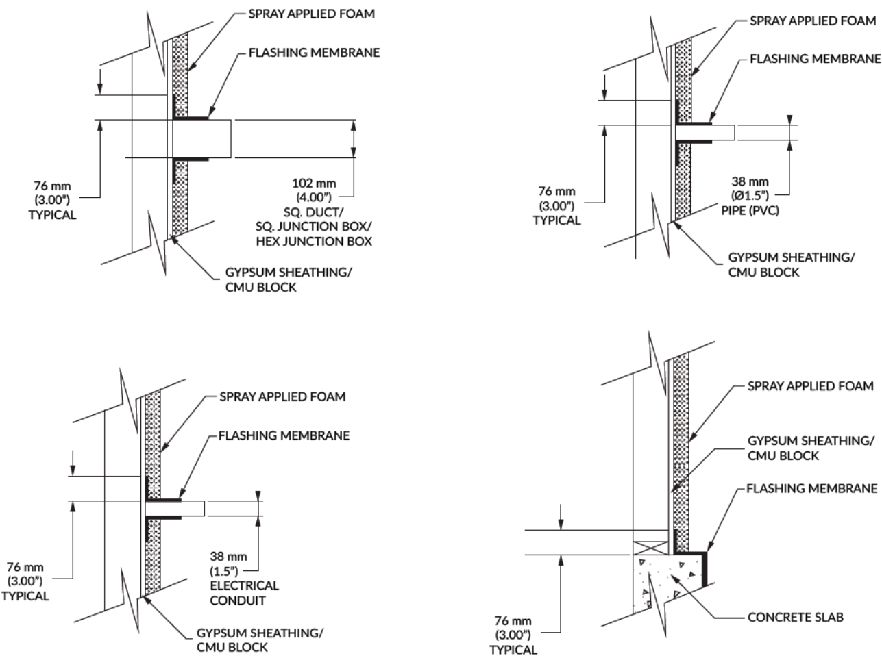
Figure 7. Penetration details
